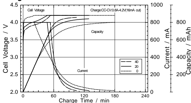
Charge characteristics
